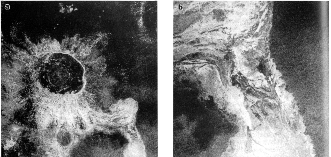
Figure 13. The second largest crater seen to date on Venus, Isabella (30°S,201°E; diameter 175 km). Magellan full-resolution radar images. ( a ) Overview, showing dark floor with concentric fractures and vague domical uplift but no central peak feature and large outflow complex to south and southeast. Note channel and drainage delta layout of large outflow to southeast. ( b ) Close-up of large outflow to southeast, showing complex, anastomosing multiple channel morphology and drain-out region. Width of field 115 km.
