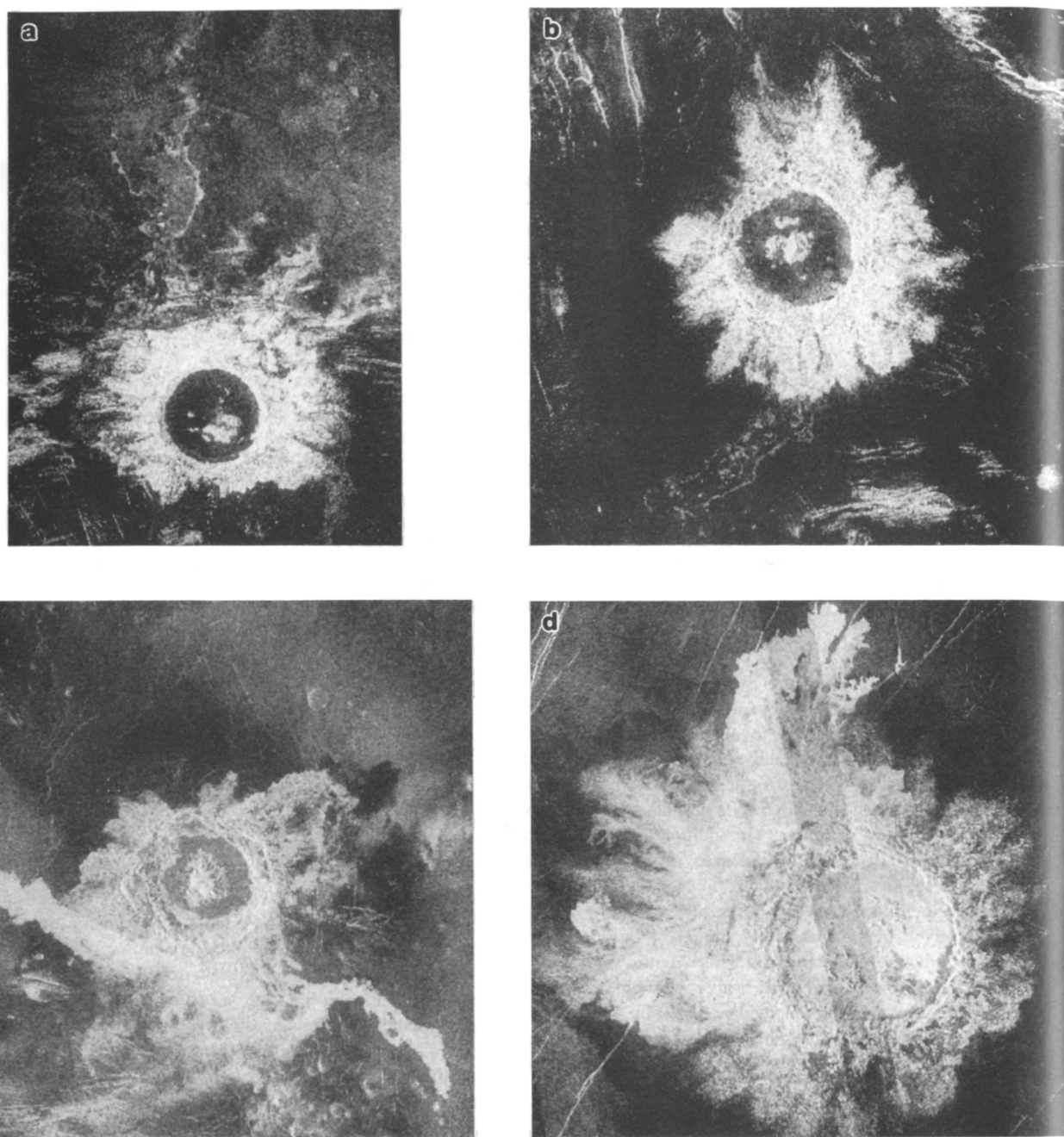
Figure 1. Full-resolution Magellan radar images of impact craters on Venus. In all Magellan radar images, north is up, and illumination is from the west. (a) Aglaonice ( 26.2^{\circ}\text{S} , 339.7^{\circ}\text{E} ; diameter 63 km), with large fluid outflow to north and small outflow to southeast. (b) Danilova ( 26.6^{\circ}\text{S} , 337.2^{\circ}\text{E} ; diameter 48 km), with large outflow to south and small outflow to north. (c) Carson ( 24^{\circ}\text{S} , 343^{\circ}\text{E} ; diameter 39 km), with two bright flows originating to south and flowing to east and west. (d) Stuart ( 30^{\circ}\text{S} , 21^{\circ}\text{E} ; diameter 67 km).
