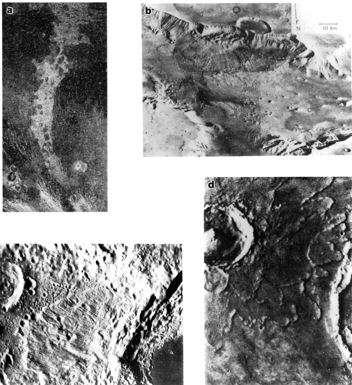
Figure 2. Examples of deposits left by flow processes. (a) Magellan radar image of lava flow from large volcano Sif Mons, at 7^{\circ}\text{N} , 350^{\circ}\text{E} . Width of frame 154 km. (b) Viking orbiter mosaic 14A27-32, showing large avalanche deposit from wall of Valles Marineris on Mars, extending across valley floor. Scale shown. (c) Apollo 17 orbiter frame M-2608, showing large avalanche deposit from rim of farside crater Tsiolkovsky. Lineated avalanche deposit is about 80 km long. (d) Viking orbiter mosaic 3A07, showing impact crater Yuty (diameter 19 km) on Mars with characteristic fluidized ejecta blanket, including outer rampart and multiple flow lobes.
