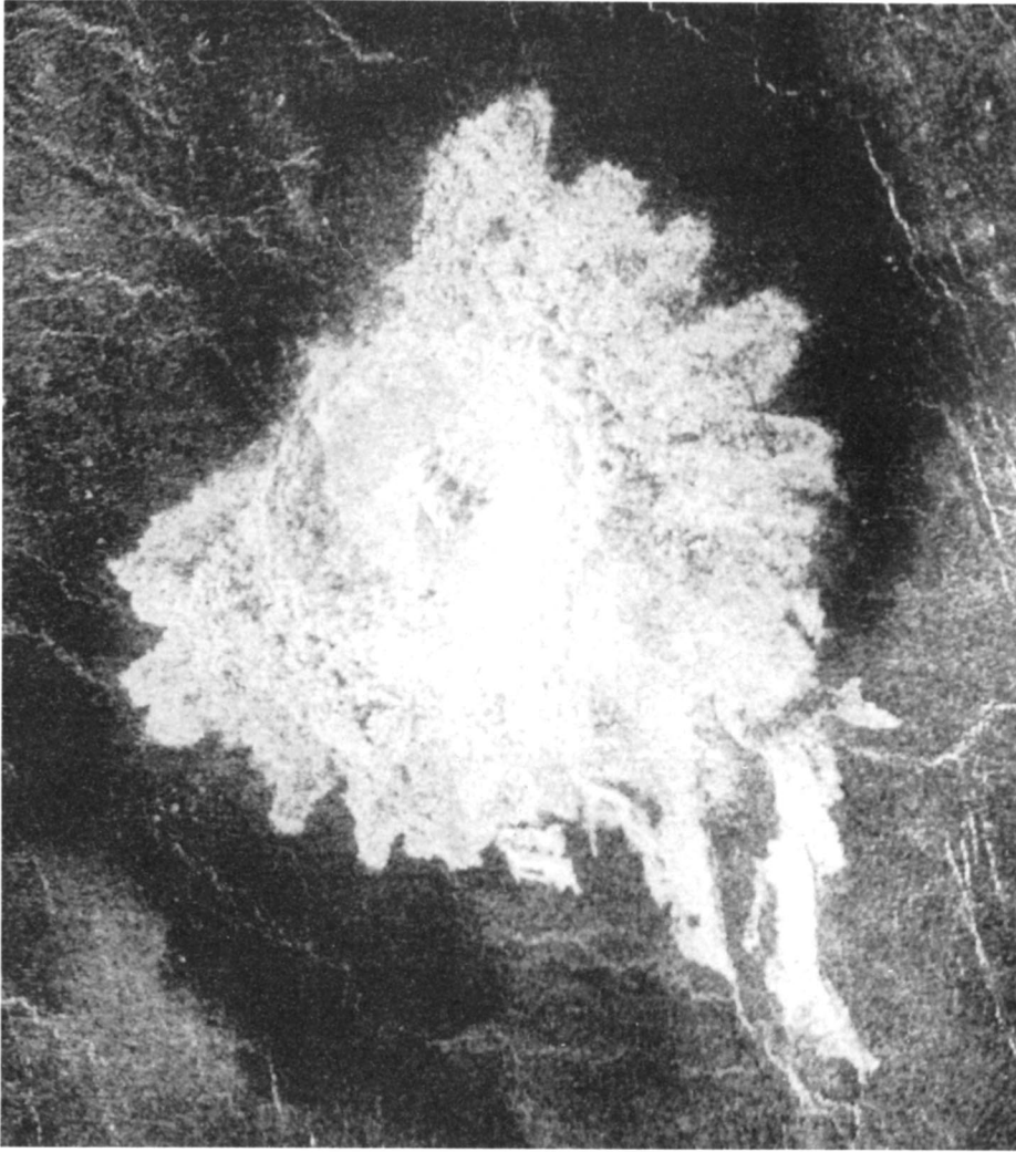
Figure 3. Magellan full-resolution radar image of crater Aurelia (20.3°N,331.8°E; diameter 31 km). Note standard elements of crater deposits on Venus: central peak, flat floor, terraced inner walls, sharp topographic rim, hummocky inner ejecta, lobate-edged outer continuous ejecta, dark halo on surrounding plains, and outflows to southeast. Note missing sector of ejecta to northwest.
