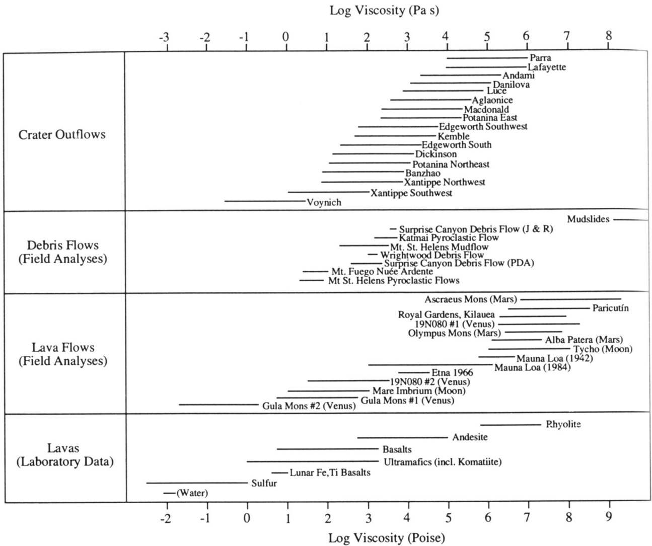
Figure 15. Results for viscosity analyses of 17 Venus crater outflows and reference viscosity measurements from field analyses of various debris flows and lava flows elsewhere in the solar system and laboratory analyses of magmas of several compositions. Citations for values from literature are in text. Lines represent estimated error ranges.
